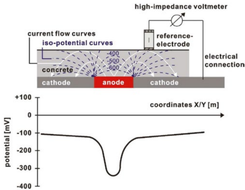
Figure 3: Measuring principle.
